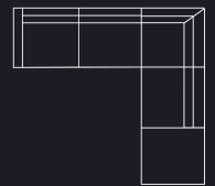
3 seater + corner 90 + 1.5 seater + footstool with storage (R)* H96 x D244 x W287cm
